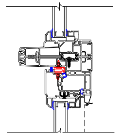
Modular Mullion (with optional reinforcement shown)
