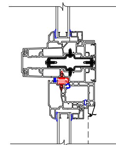
Modular Mullion (with optional 5/8" reinforcement shown)
