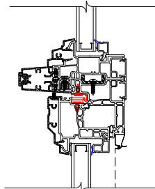
Modular Mullion (with optional reinforcement shown)
