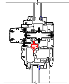
Modular Mullion (with optional 5/8" reinforcement shown)
