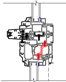
Modular Mullion (with optional reinforcement shown)
