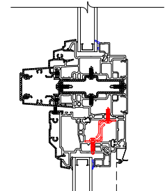
Modular Mullion (with optional 5/8" reinforcement shown)
