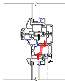
Modular Mullion (with optional reinforcement shown)
